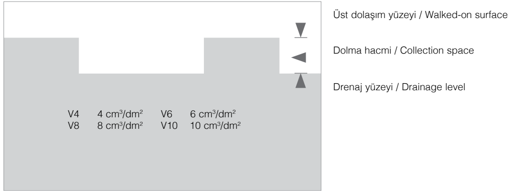
Karo kesiti / Cross-section of tile
